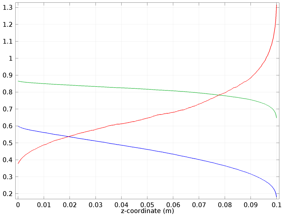
Line Graph: p2/Pin (1) Line Graph: T/(273.15[K]) (1) Line Graph: Mach number (1)
