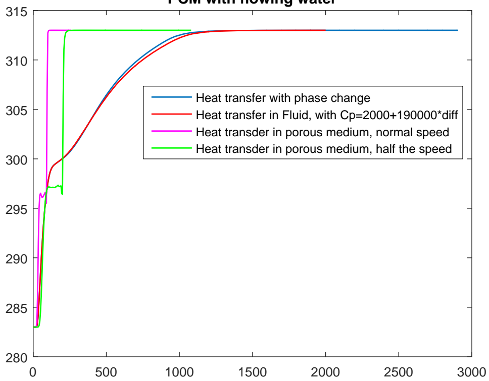
PCM with flowing water
