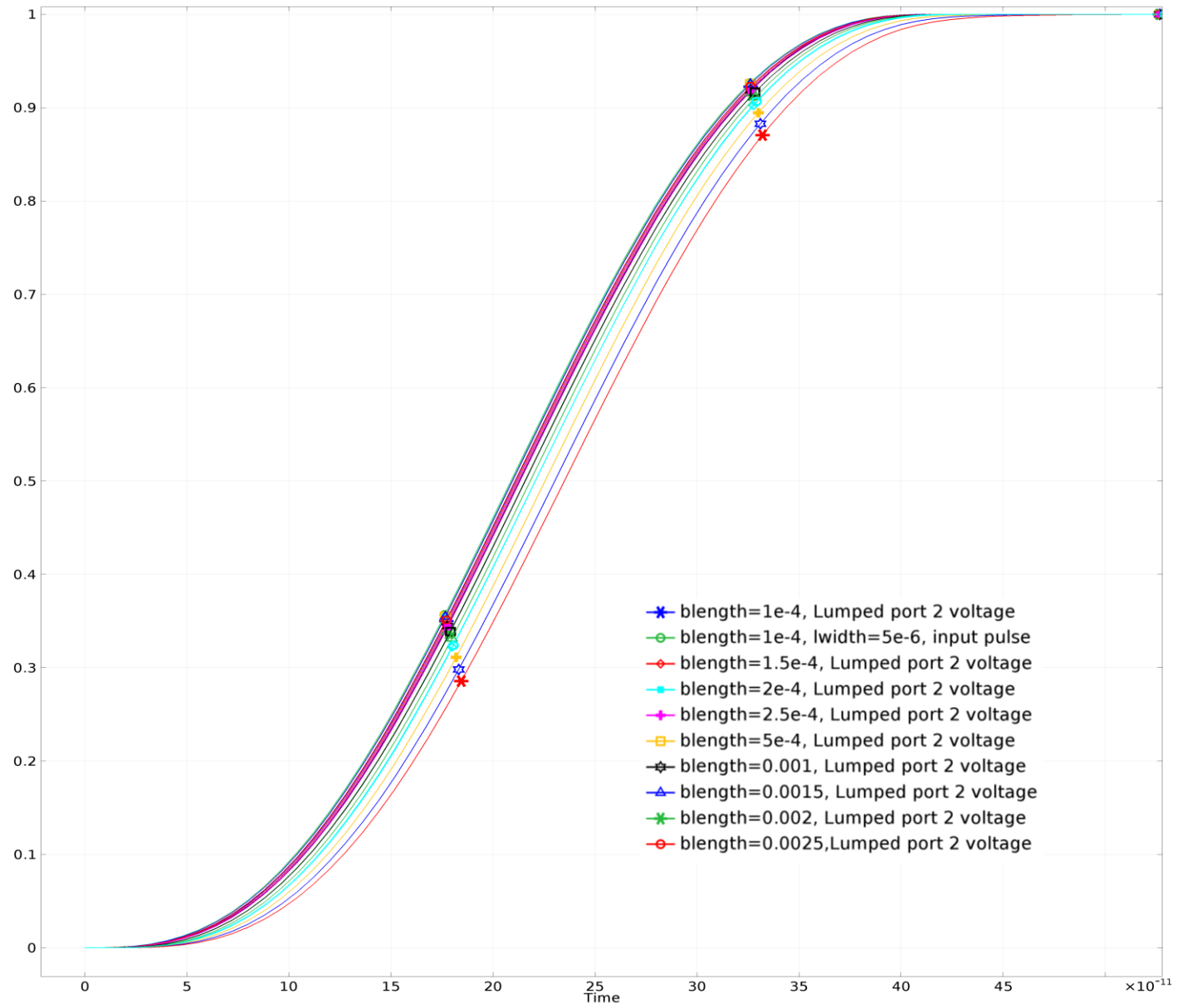
Time domain response at the through port
