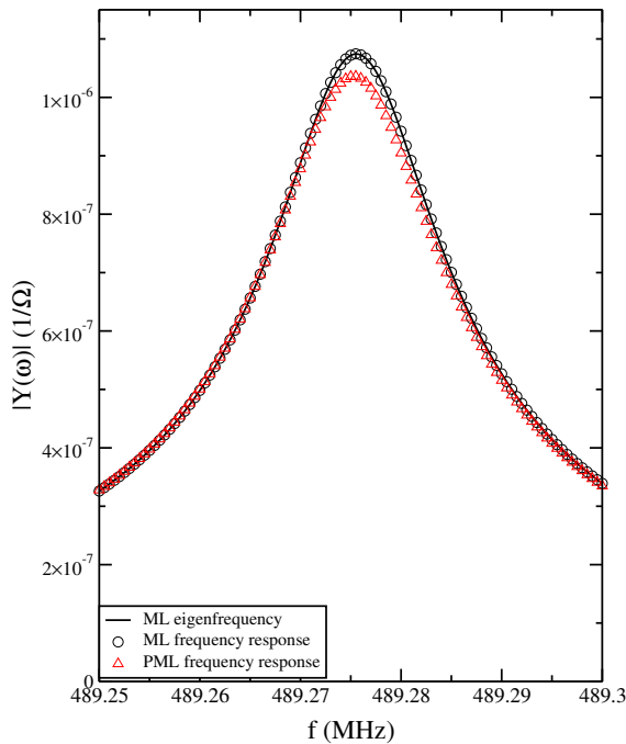
Figure 7 Admittance of the first radial bulk-mode of the diamond disk resonator with R=11 \mu\text{m} and a=0.8 \mu\text{m} . Equation (8) with ML is compared to the frequency response mode analysis with ML and PML. V_{ac}=2.5\text{V} , g=90 \text{ nm} [1].
